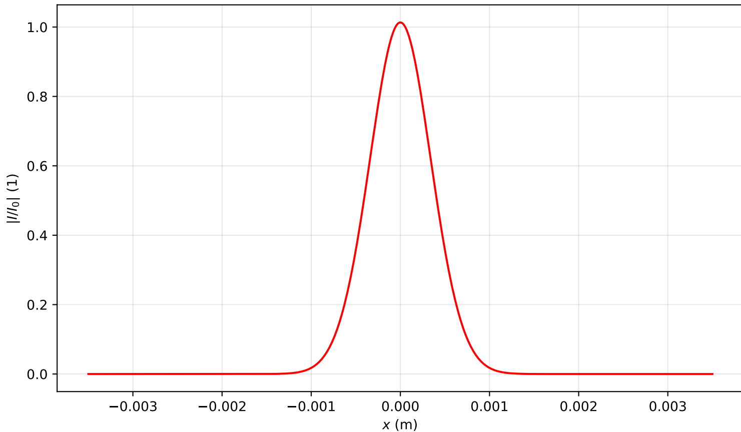
Intensity profile I(x, y = 0, z = 0.239)/I_0 , P_{in}=0.5P_{cr} , artificial time
